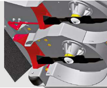
A REAR DISCHARGE CUT CUTTING CHAMBER OPEN
