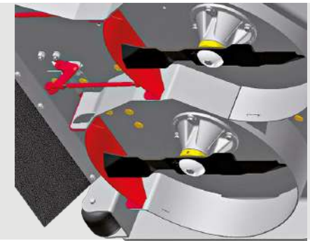
B MULCHING CUT CUTTING CHAMBER CLOSED
